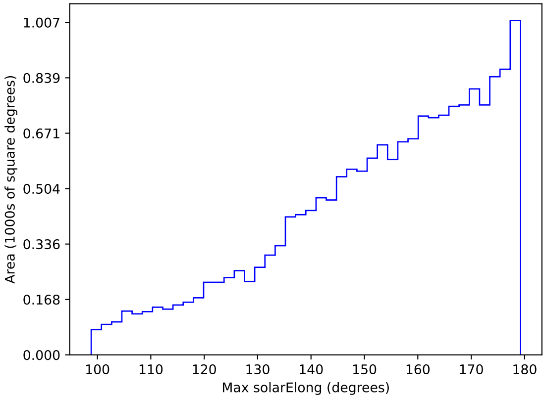
too_elab_r8_d2_griz_v3.4_10yrs WFD y band: Max solarElong
