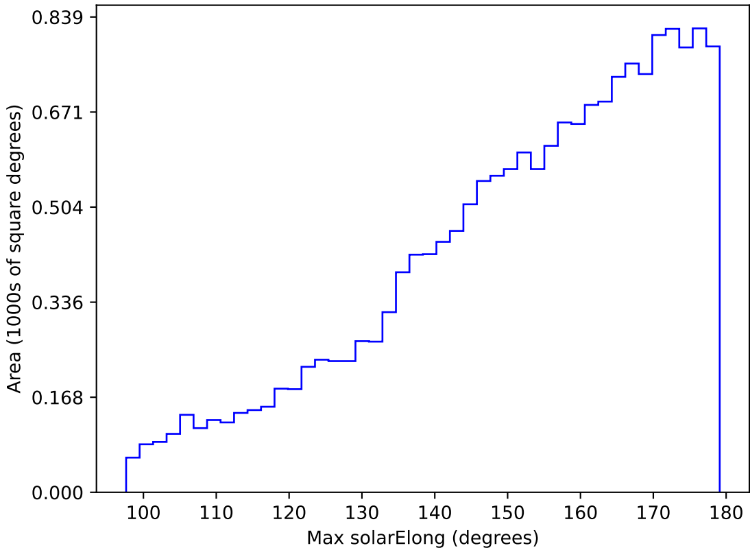
too_elab_r8_d2_griz_v3.4_10yrs WFD u band: Max solarElong
