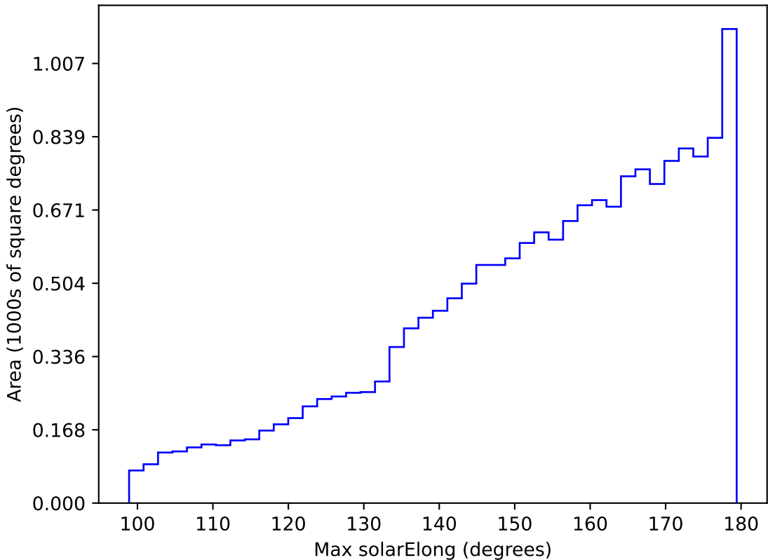
too_elab_r8_d2_griz_v3.4_10yrs WFD r band: Max solarElong
