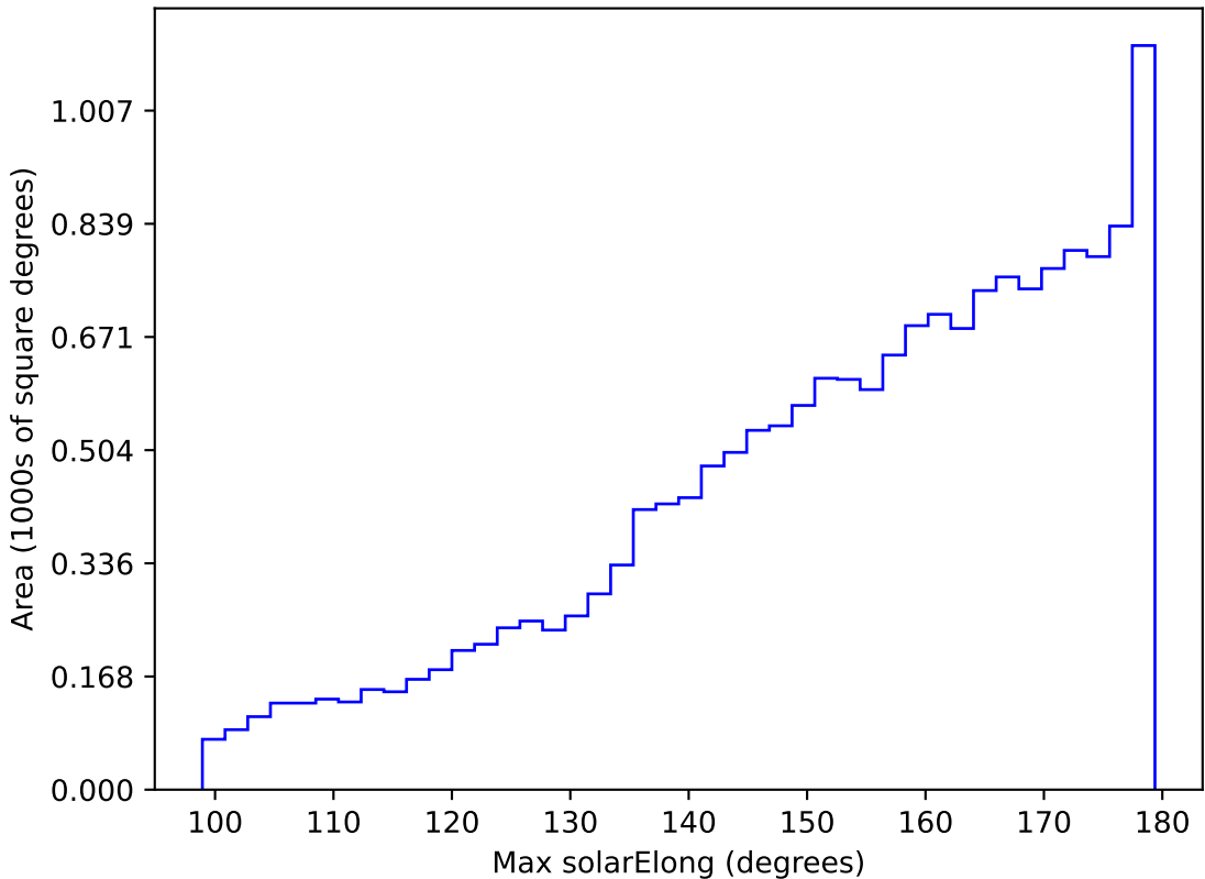
too_elab_r8_d2_griz_v3.4_10yrs WFD i band: Max solarElong
