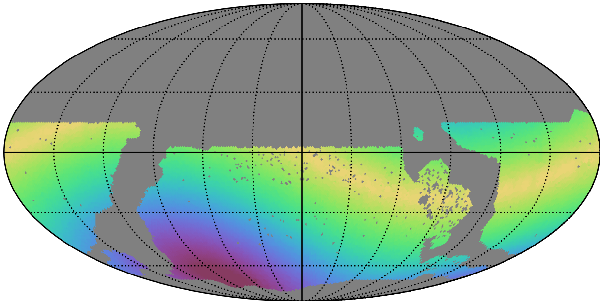
too_elab_r8_d2_griz_v3.4_10yrs WFD g band: Max solarElong
