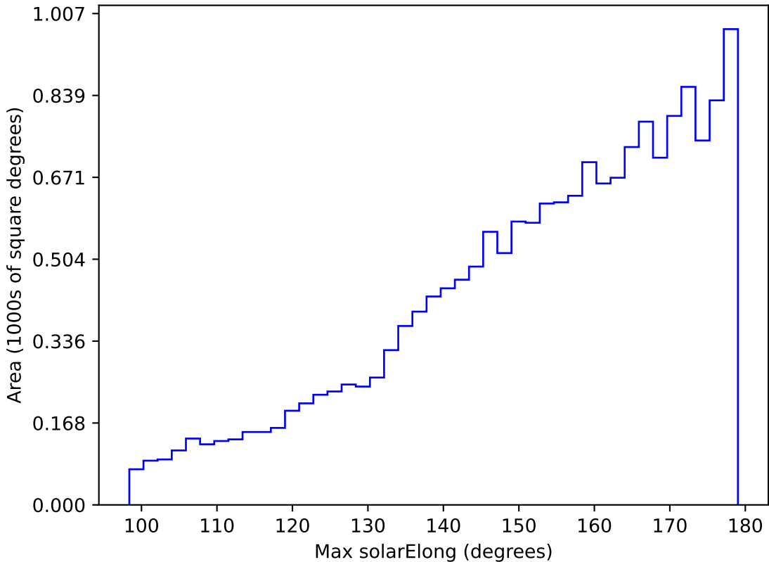
too_elab_r8_d2_griz_v3.4_10yrs WFD g band: Max solarElong
