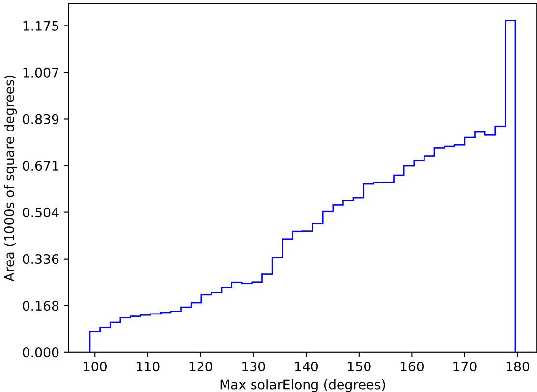
too_elab_r8_d2_griz_v3.4_10yrs WFD all bands: Max solarElong
