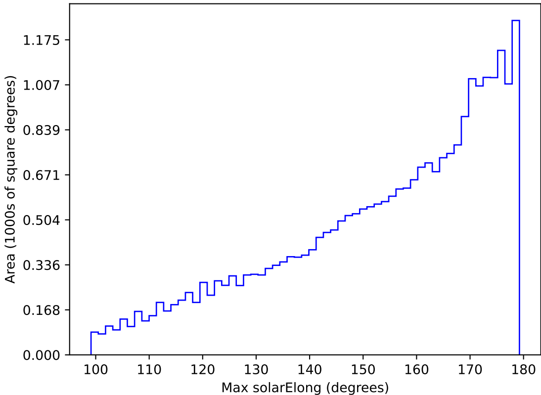
too_elab_r8_d2_griz_v3.4_10yrs All sky z band: Max solarElong
