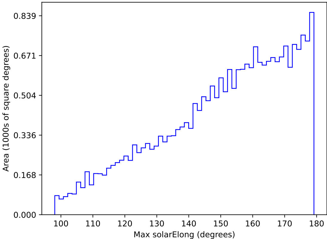
too_elab_r8_d2_griz_v3.4_10yrs All sky y band: Max solarElong
