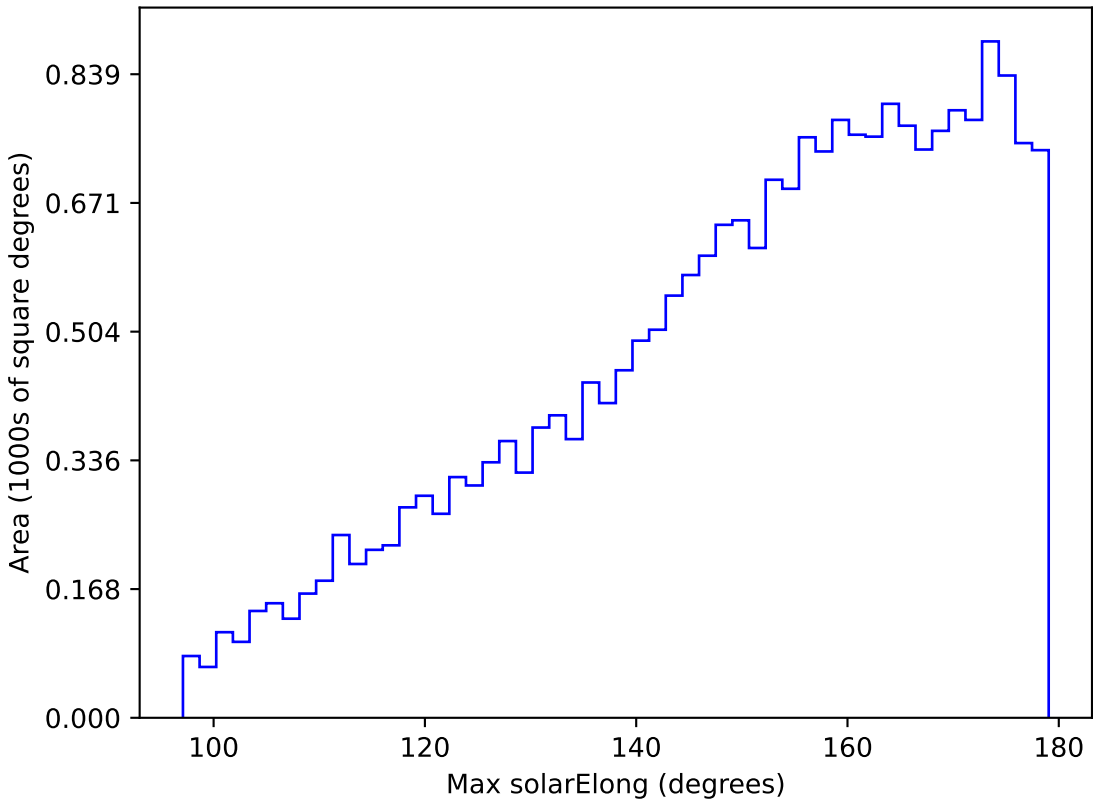
too_elab_r8_d2_griz_v3.4_10yrs All sky u band: Max solarElong
