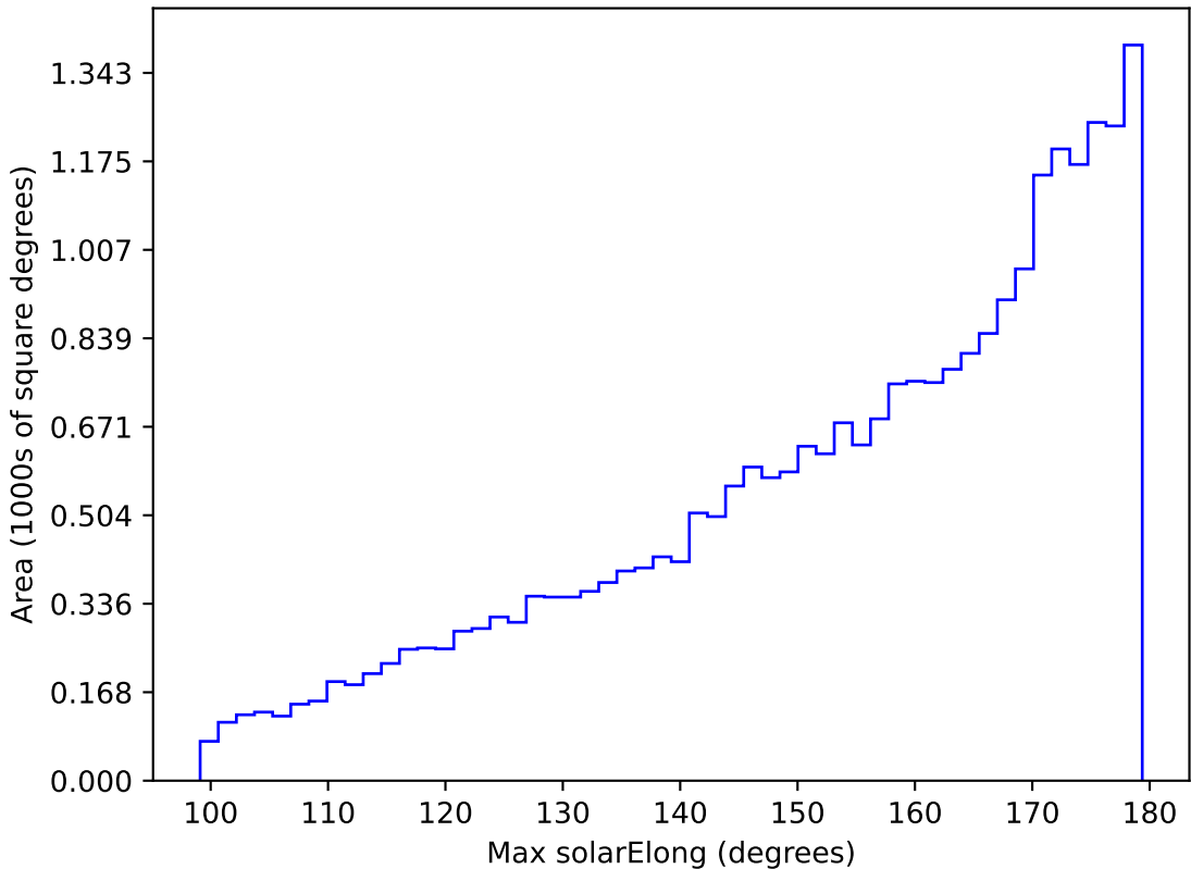
too_elab_r8_d2_griz_v3.4_10yrs All sky r band: Max solarElong
