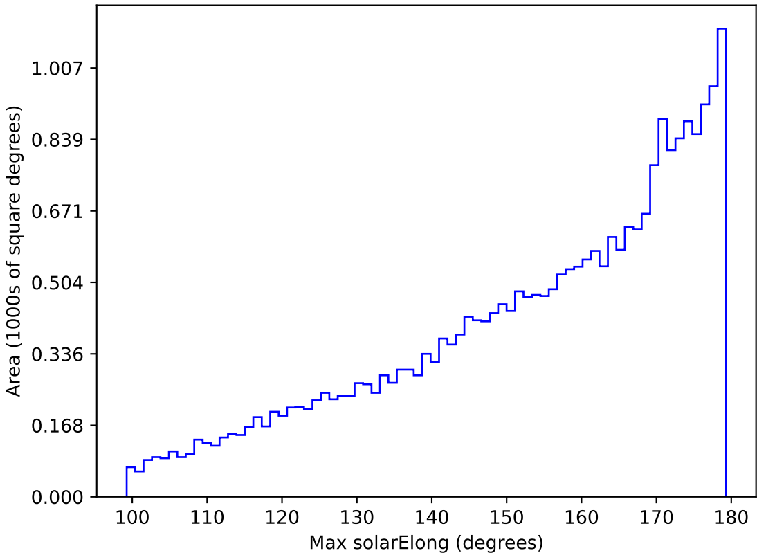
too_elab_r8_d2_griz_v3.4_10yrs All sky i band: Max solarElong
