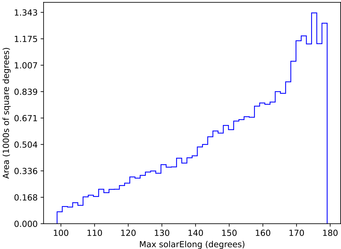
too_elab_r8_d2_griz_v3.4_10yrs All sky g band: Max solarElong
