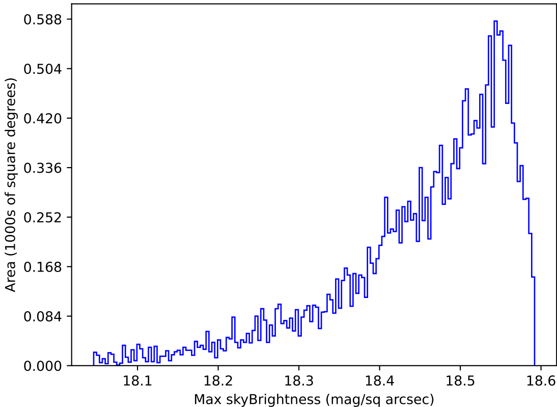
too_elab_r8_d2_griz_v3.4_10yrs Yr 1 y band: Max skyBrightness
