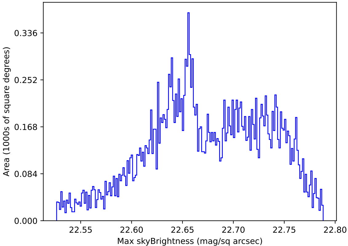
too_elab_r8_d2_griz_v3.4_10yrs Yr 1 u band: Max skyBrightness
