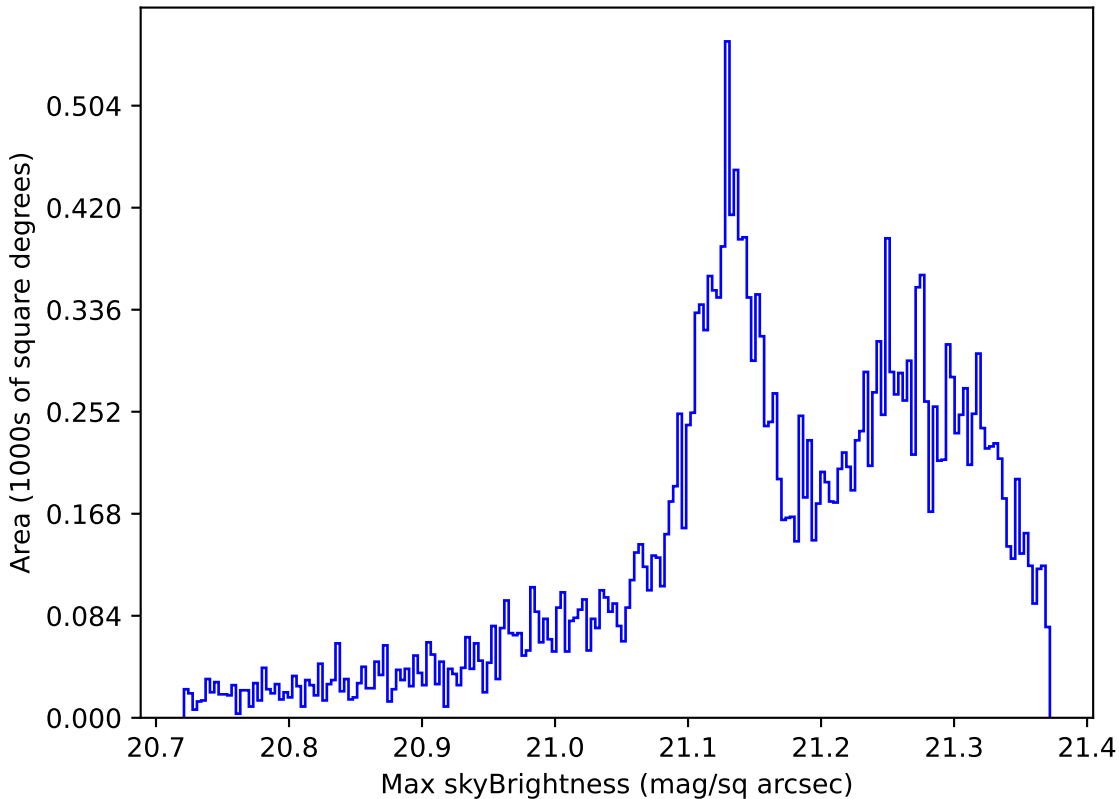
too_elab_r8_d2_griz_v3.4_10yrs Yr 1 r band: Max skyBrightness
