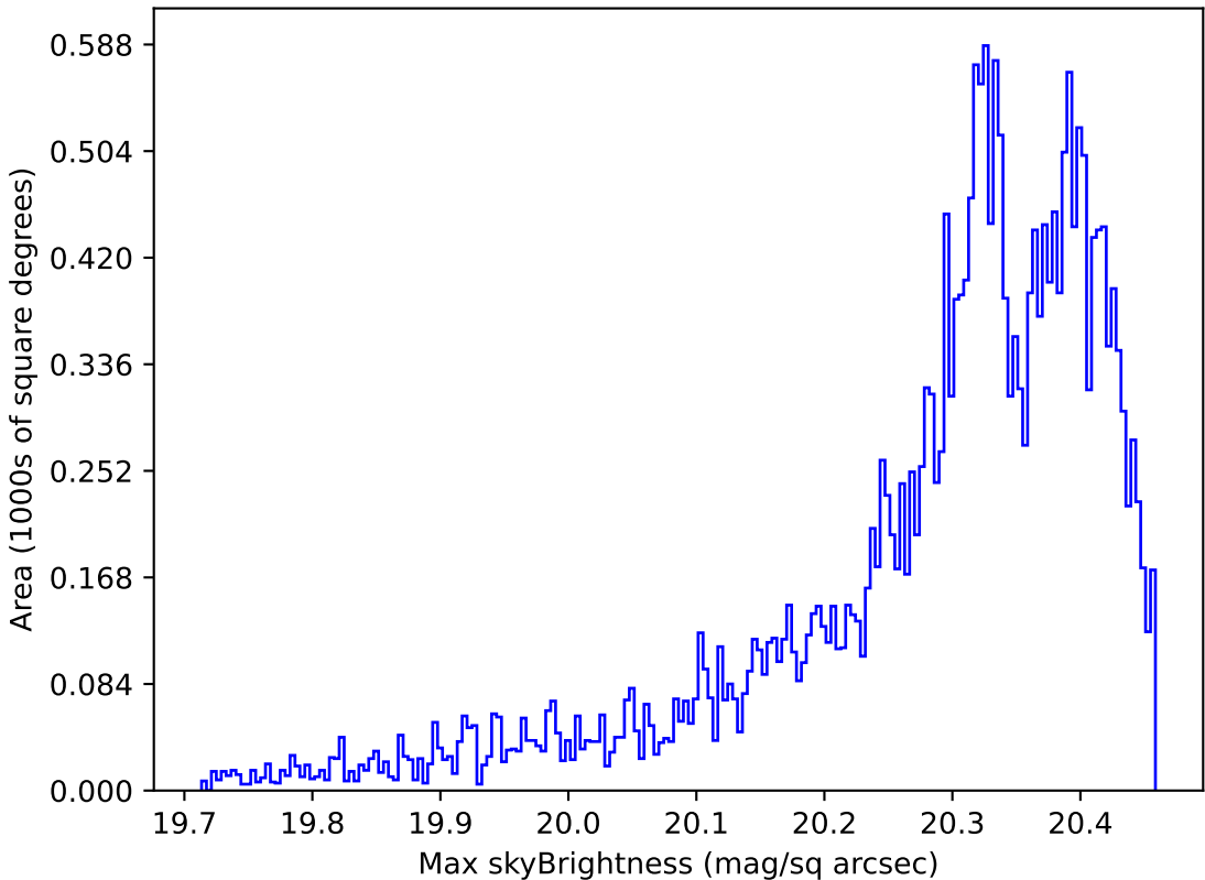
too_elab_r8_d2_griz_v3.4_10yrs Yr 1 i band: Max skyBrightness
