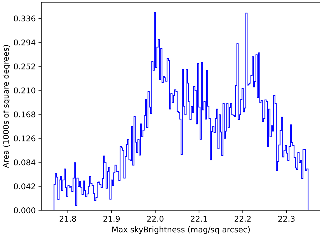
too_elab_r8_d2_griz_v3.4_10yrs Yr 1 g band: Max skyBrightness
