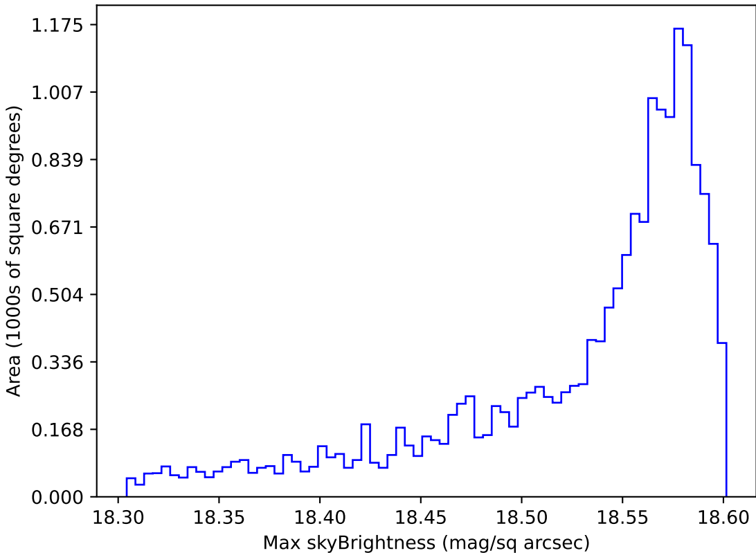
too_elab_r8_d2_griz_v3.4_10yrs WFD y band: Max skyBrightness
