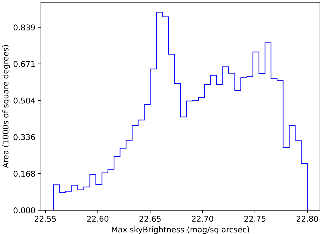
too_elab_r8_d2_griz_v3.4_10yrs WFD u band: Max skyBrightness
