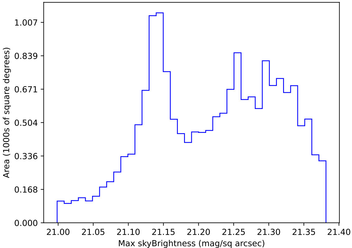
too_elab_r8_d2_griz_v3.4_10yrs WFD r band: Max skyBrightness
