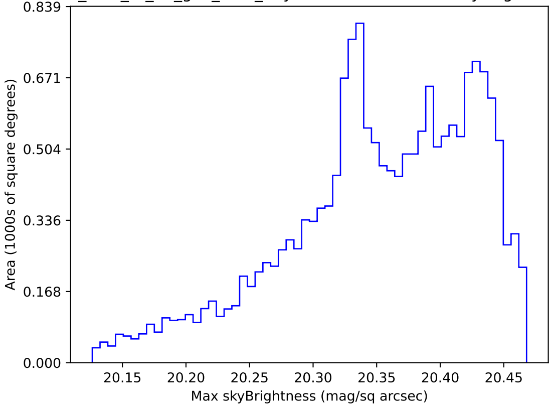
too_elab_r8_d2_griz_v3.4_10yrs WFD i band: Max skyBrightness
