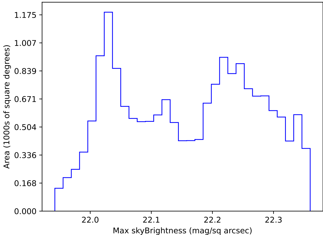
too_elab_r8_d2_griz_v3.4_10yrs WFD g band: Max skyBrightness
