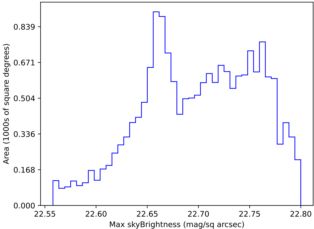
too_elab_r8_d2_griz_v3.4_10yrs WFD all bands: Max skyBrightness
