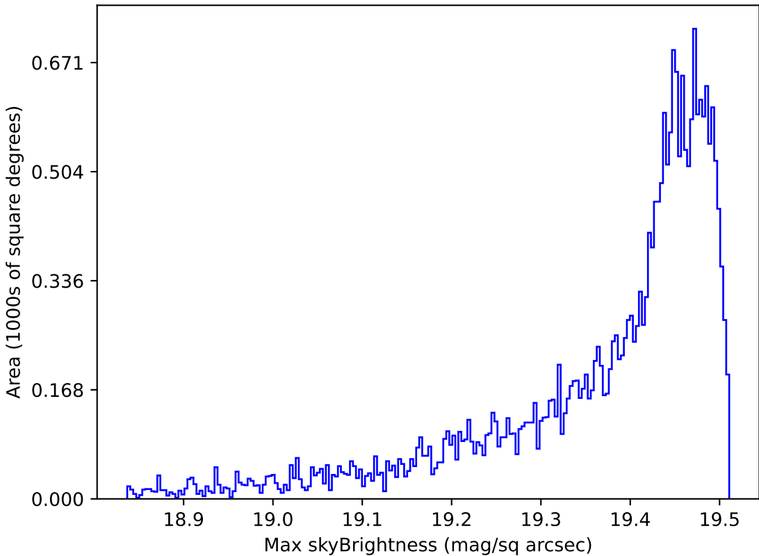
too_elab_r8_d2_griz_v3.4_10yrs All sky z band: Max skyBrightness
