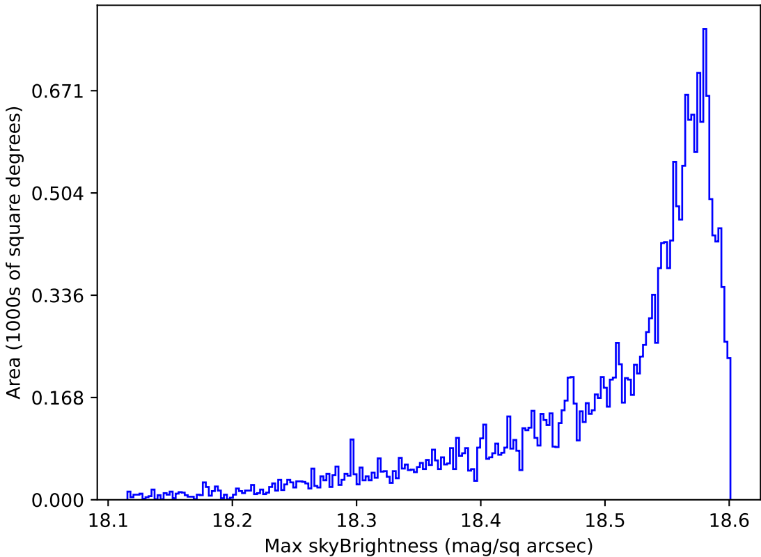
too_elab_r8_d2_griz_v3.4_10yrs All sky y band: Max skyBrightness
