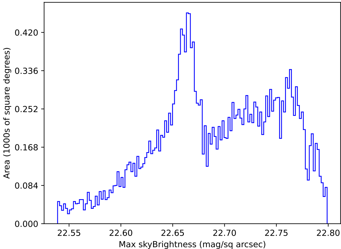
too_elab_r8_d2_griz_v3.4_10yrs All sky u band: Max skyBrightness
