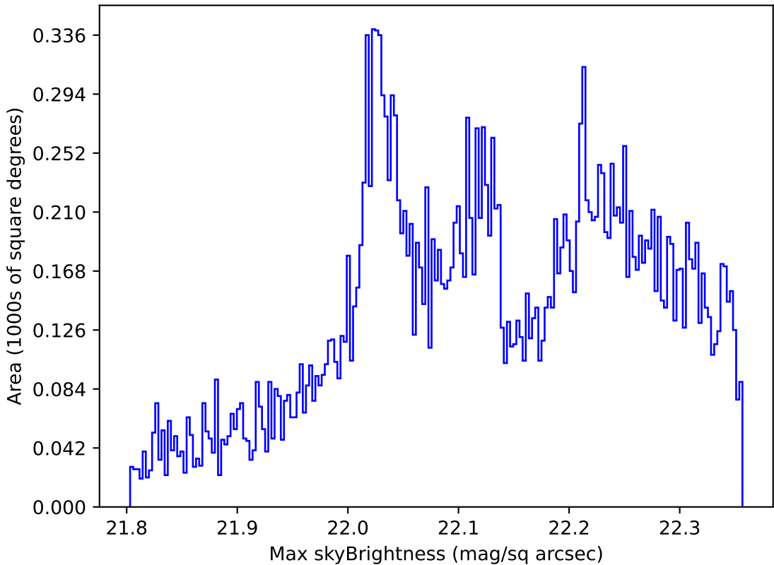
too_elab_r8_d2_griz_v3.4_10yrs All sky g band: Max skyBrightness
