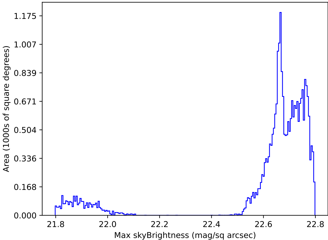
too_elab_r8_d2_griz_v3.4_10yrs All sky all bands: Max skyBrightness
