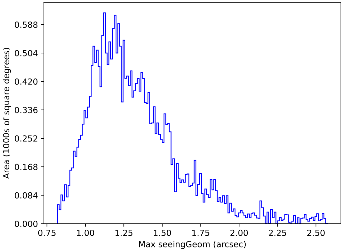
too_elab_r8_d2_griz_v3.4_10yrs Yr 1 z band: Max seeingGeom
