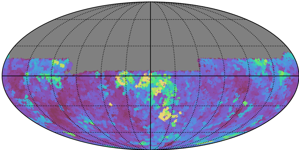
too_elab_r8_d2_griz_v3.4_10yrs Yr 1 y band: Max seeingGeom
