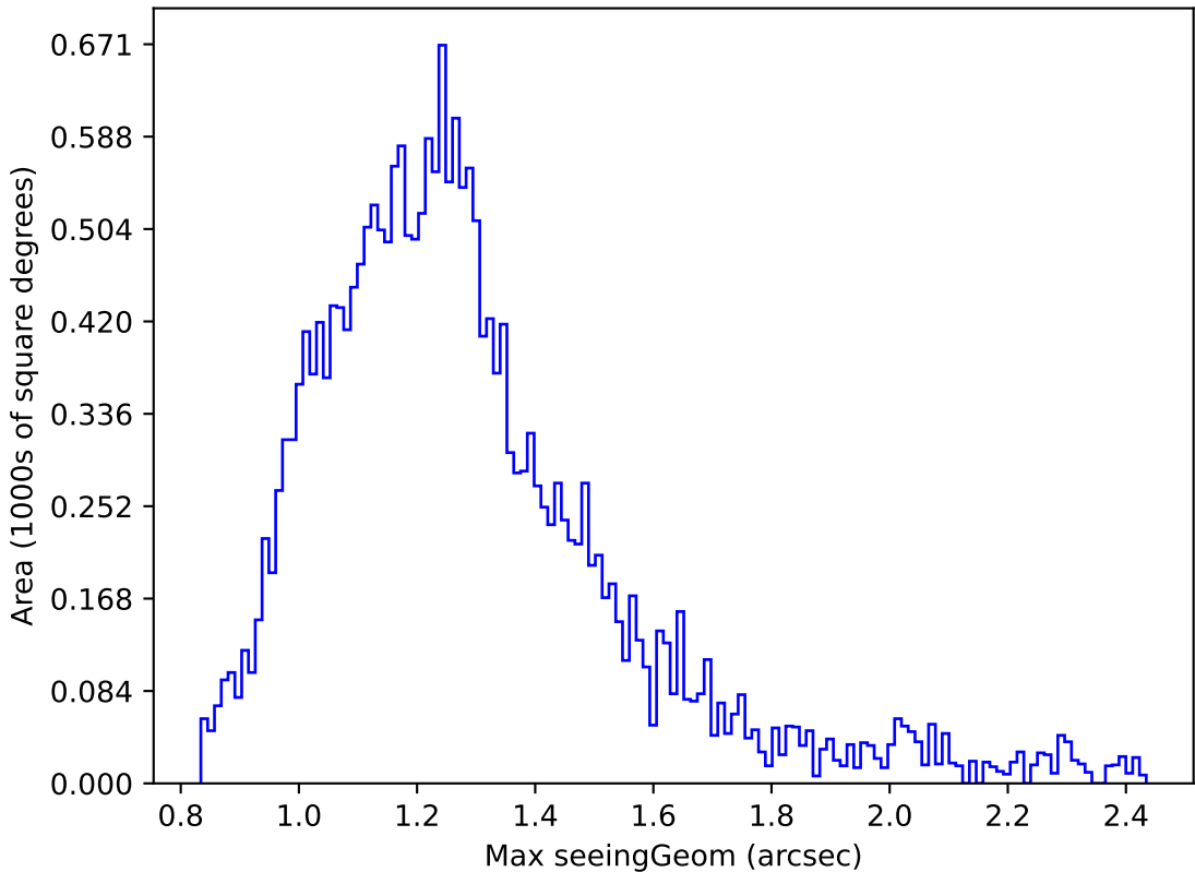
too_elab_r8_d2_griz_v3.4_10yrs Yr 1 y band: Max seeingGeom
