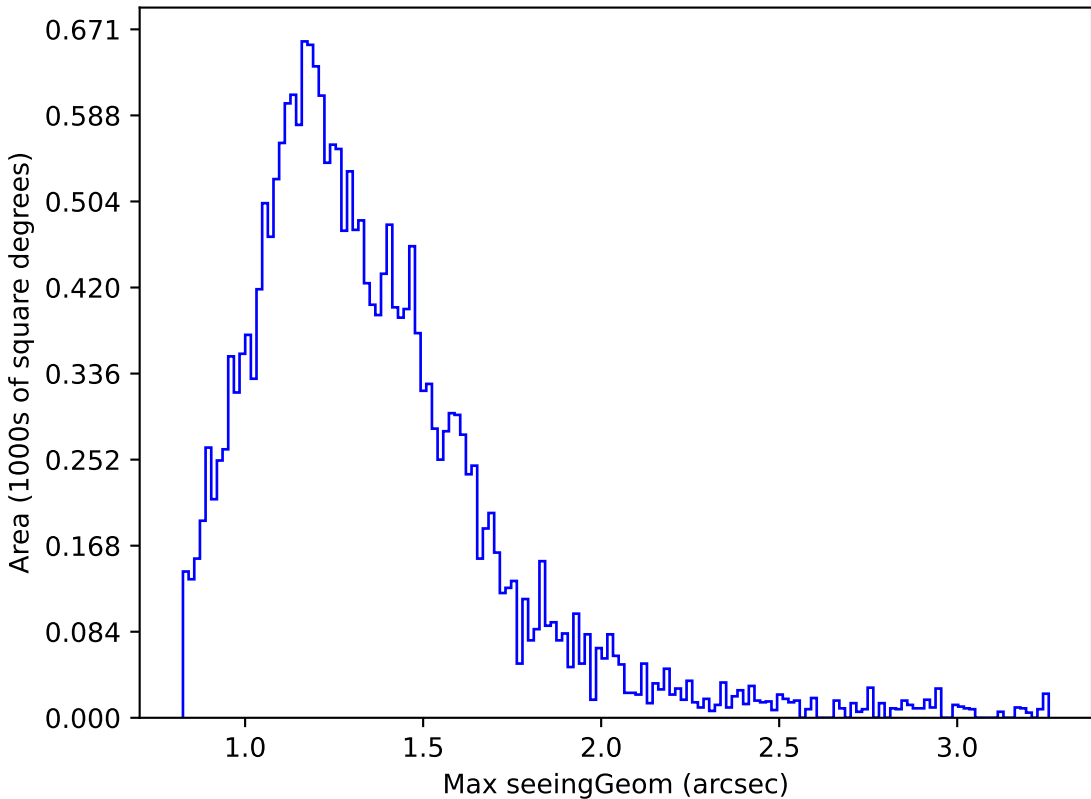
too_elab_r8_d2_griz_v3.4_10yrs Yr 1 u band: Max seeingGeom
