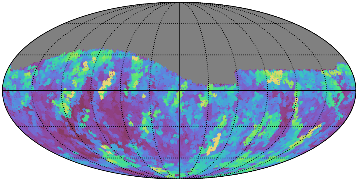
too_elab_r8_d2_griz_v3.4_10yrs Yr 1 r band: Max seeingGeom
