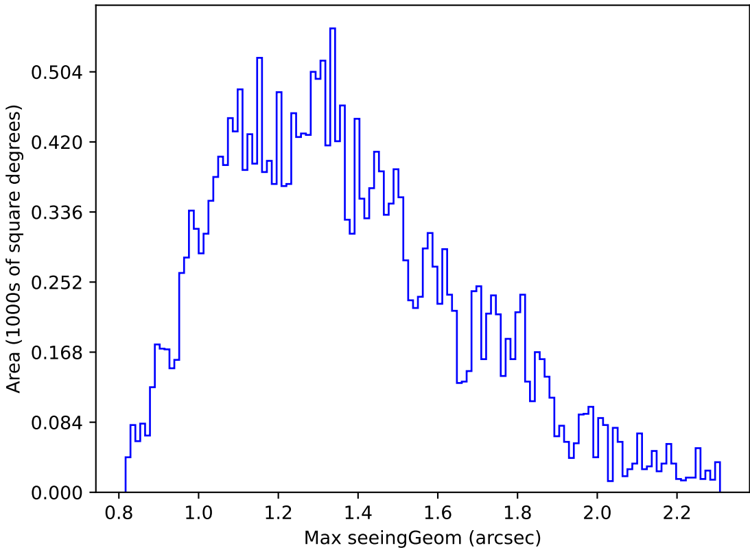
too_elab_r8_d2_griz_v3.4_10yrs Yr 1 r band: Max seeingGeom
