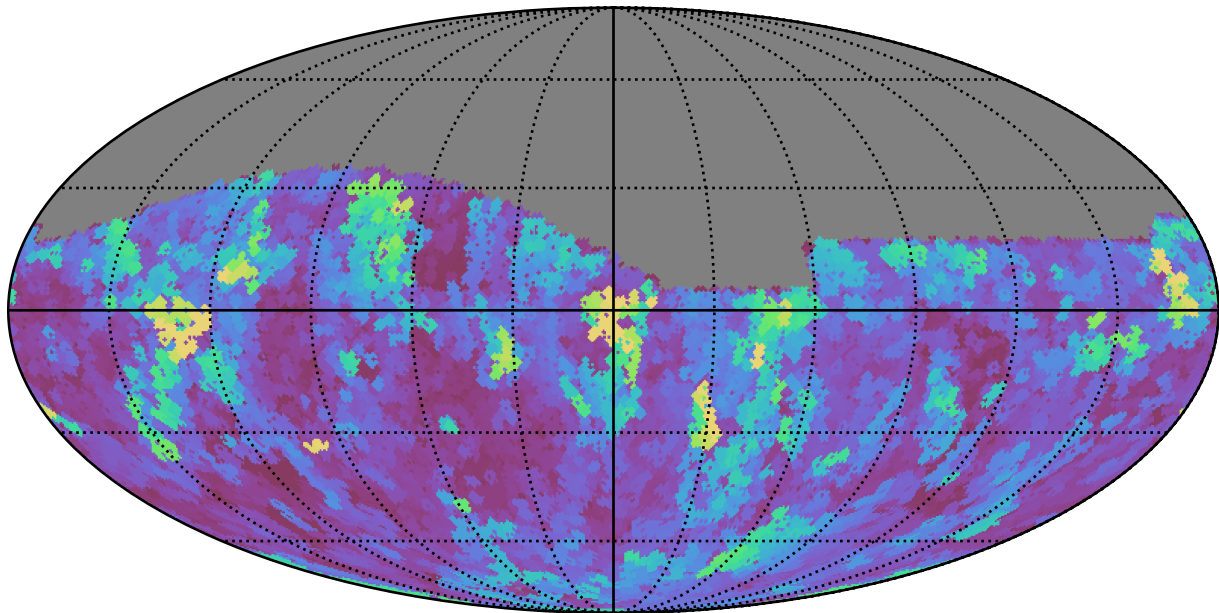
too_elab_r8_d2_griz_v3.4_10yrs Yr 1 i band: Max seeingGeom
