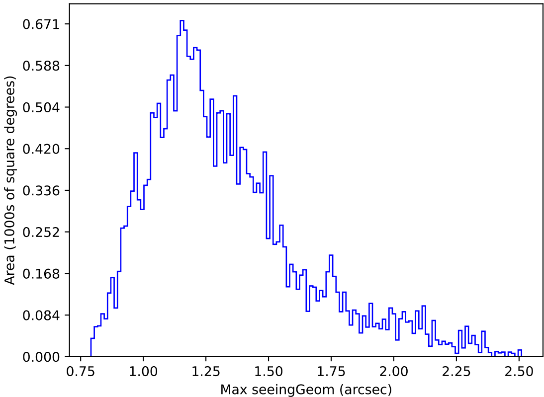
too_elab_r8_d2_griz_v3.4_10yrs Yr 1 g band: Max seeingGeom
