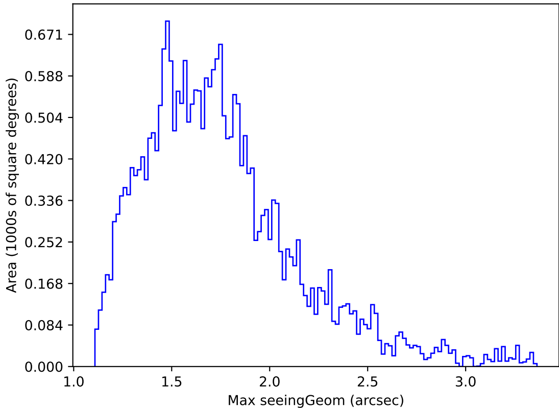
too_elab_r8_d2_griz_v3.4_10yrs Yr 1 all bands: Max seeingGeom
