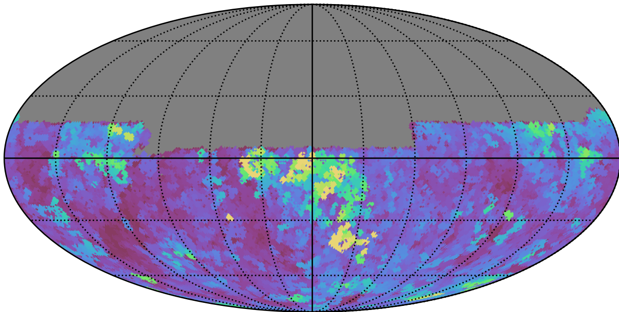
too_elab_r8_d2_griz_v3.4_10yrs Yr 1 y band: Max seeingEff
