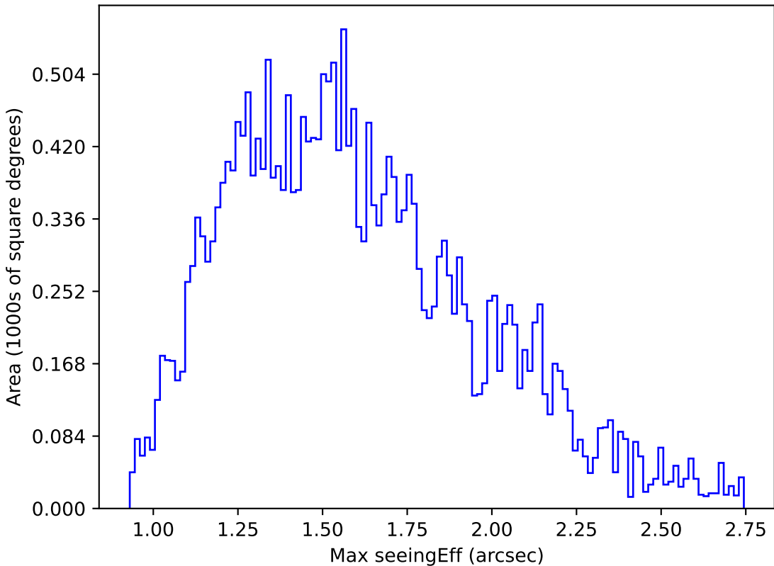
too_elab_r8_d2_griz_v3.4_10yrs Yr 1 r band: Max seeingEff
