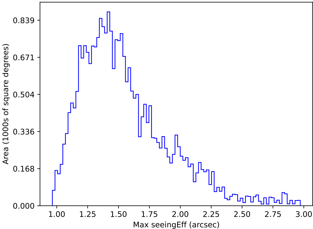
too_elab_r8_d2_griz_v3.4_10yrs Yr 1 i band: Max seeingEff
