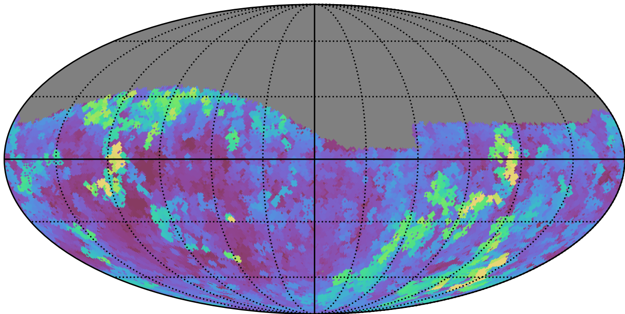
too_elab_r8_d2_griz_v3.4_10yrs Yr 1 g band: Max seeingEff
