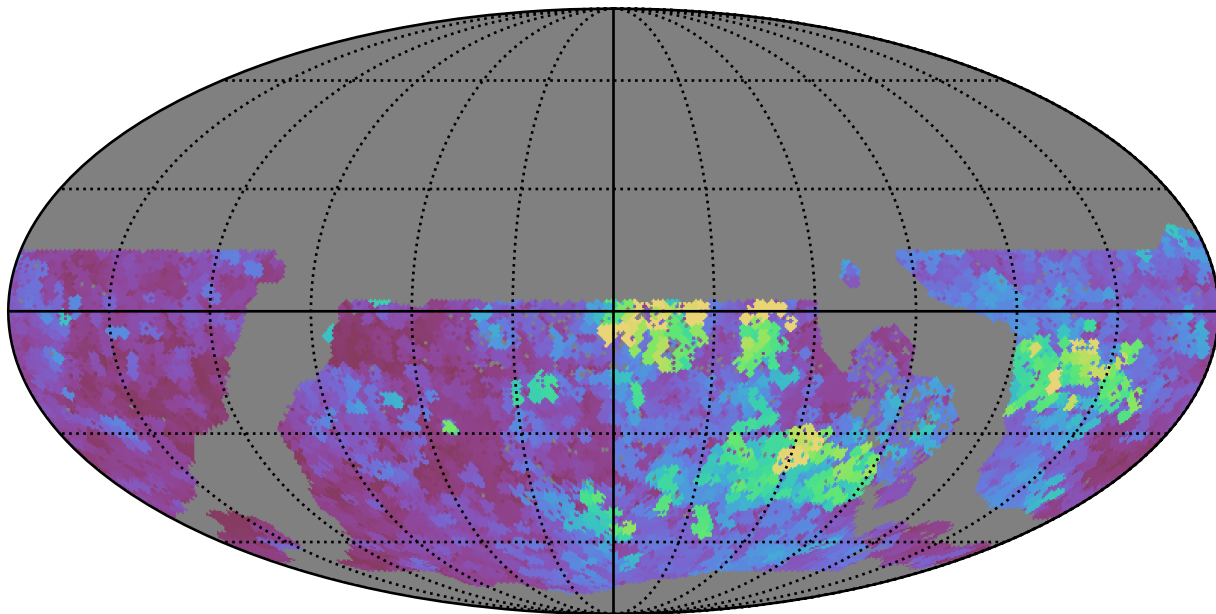
too_elab_r8_d2_griz_v3.4_10yrs WFD y band: Max seeingEff
