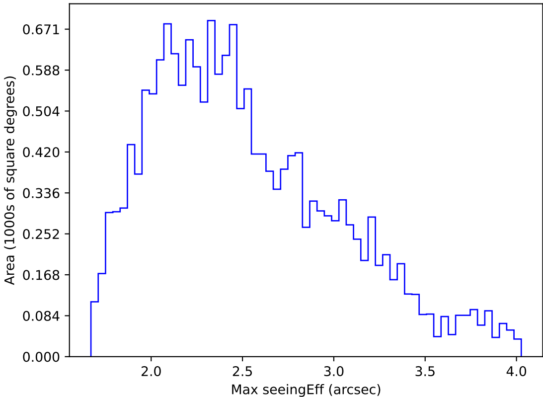
too_elab_r8_d2_griz_v3.4_10yrs WFD g band: Max seeingEff
