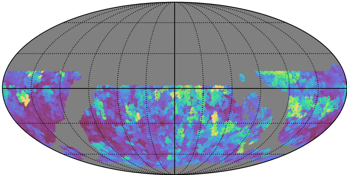
too_elab_r8_d2_griz_v3.4_10yrs WFD all bands: Max seeingEff
