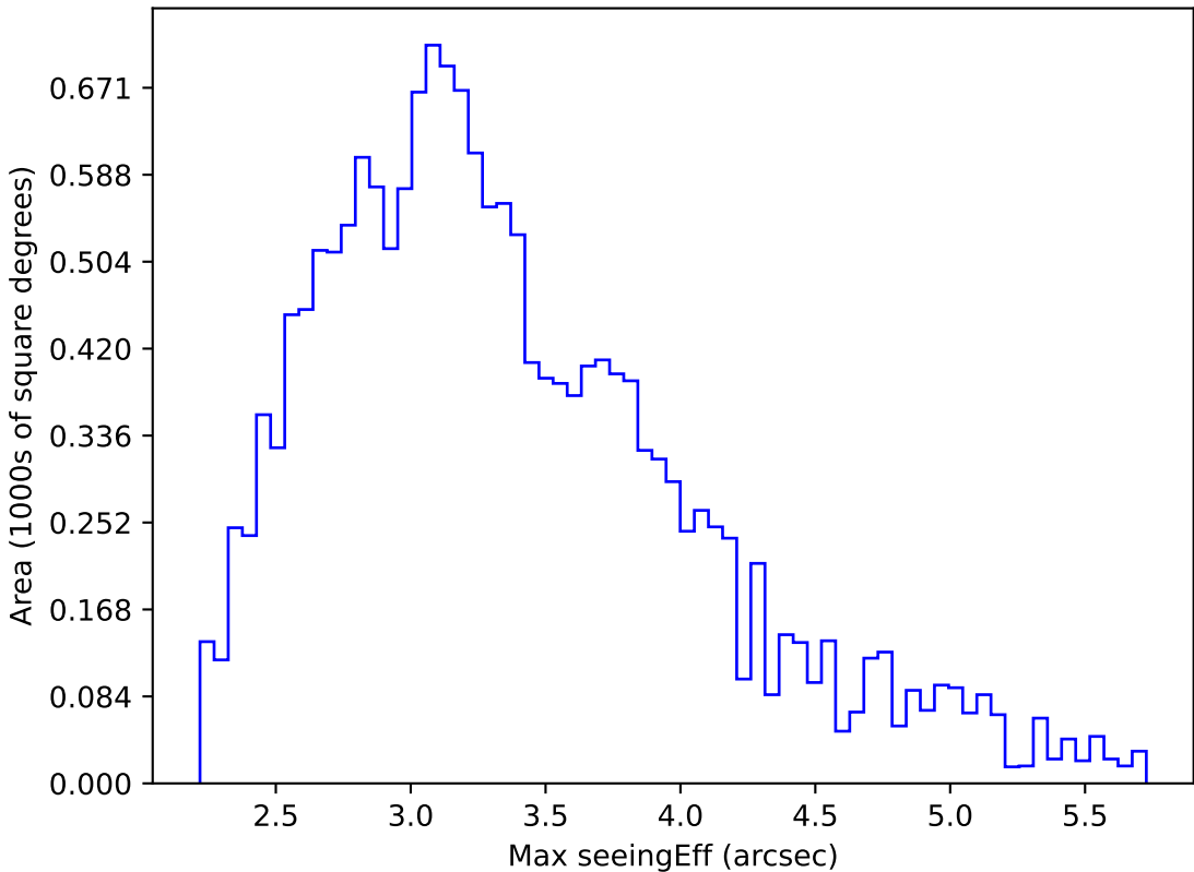
too_elab_r8_d2_griz_v3.4_10yrs WFD all bands: Max seeingEff
