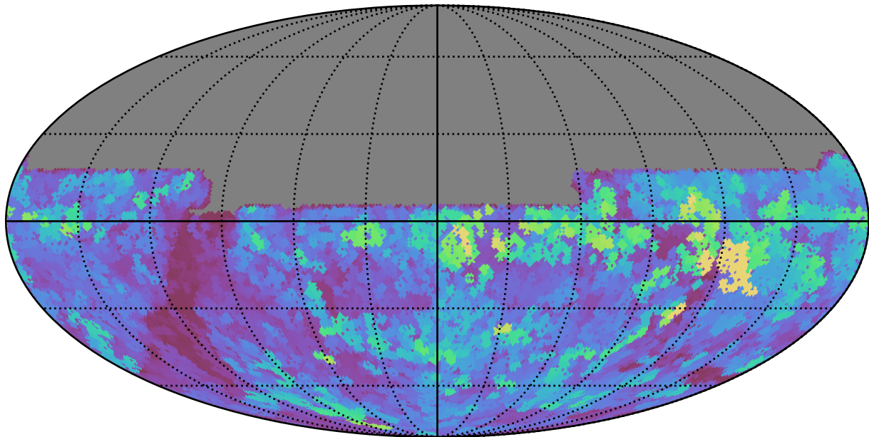
too_elab_r8_d2_griz_v3.4_10yrs All sky u band: Max seeingEff
