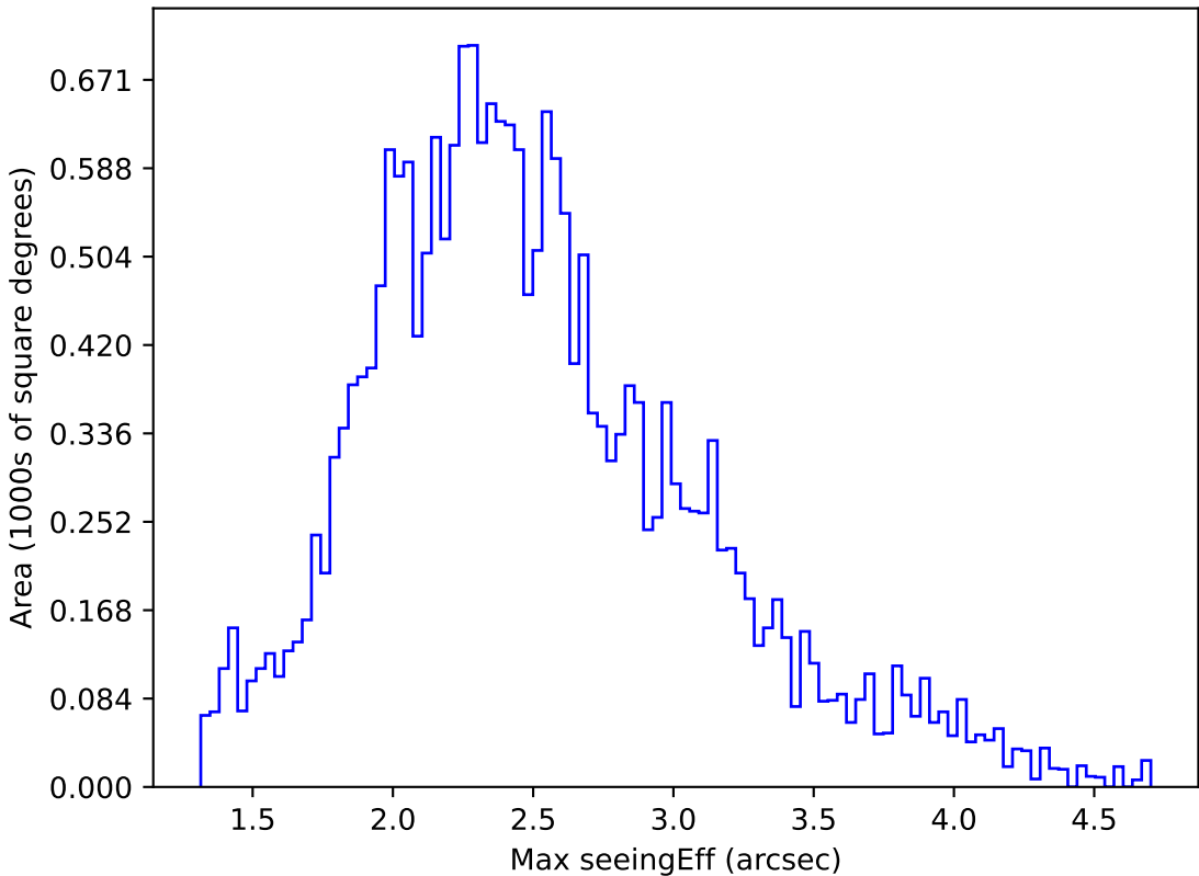
too_elab_r8_d2_griz_v3.4_10yrs All sky u band: Max seeingEff
