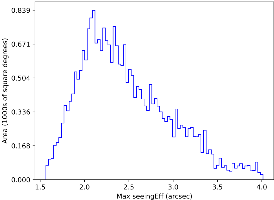
too_elab_r8_d2_griz_v3.4_10yrs All sky g band: Max seeingEff
