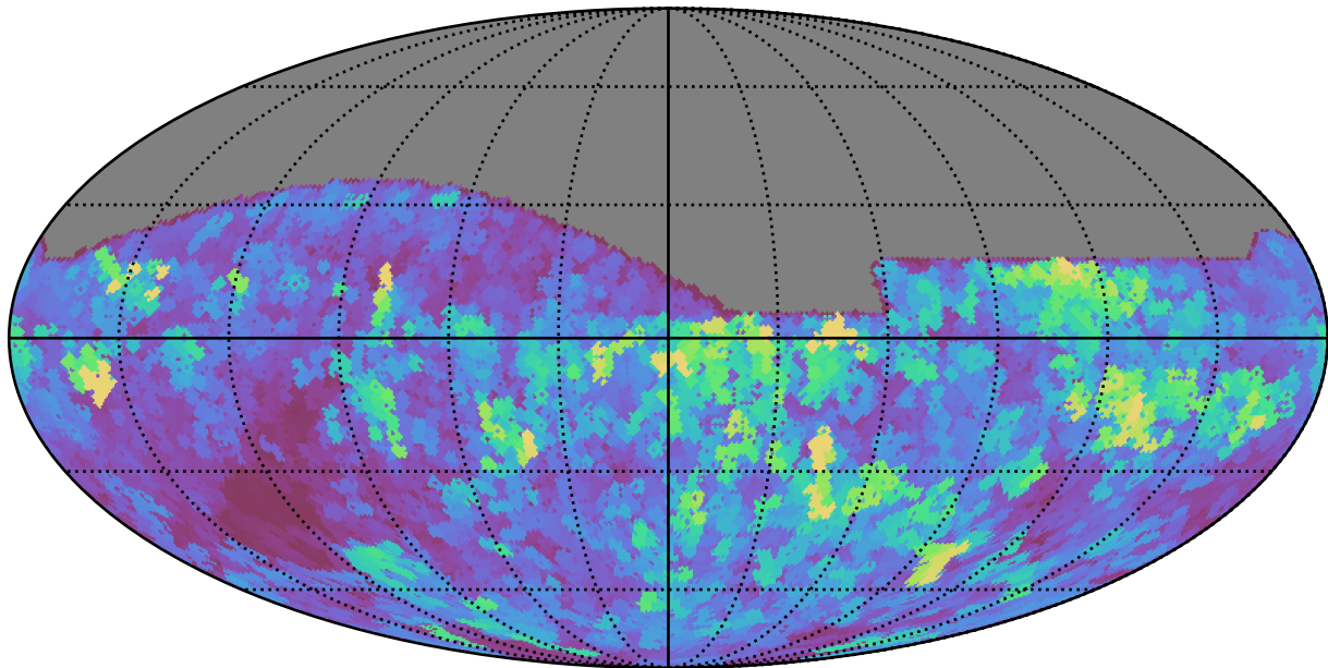
too_elab_r8_d2_griz_v3.4_10yrs All sky all bands: Max seeingEff
